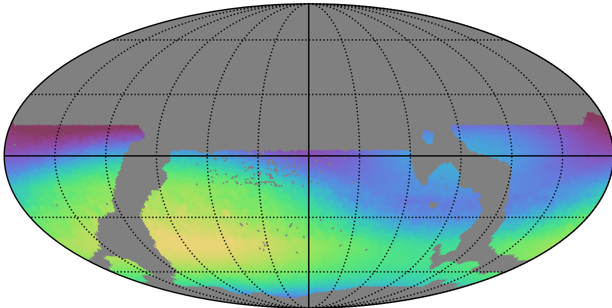
weather_cloudso30v3.4_10yrs WFD r band: Max skyBrightness
