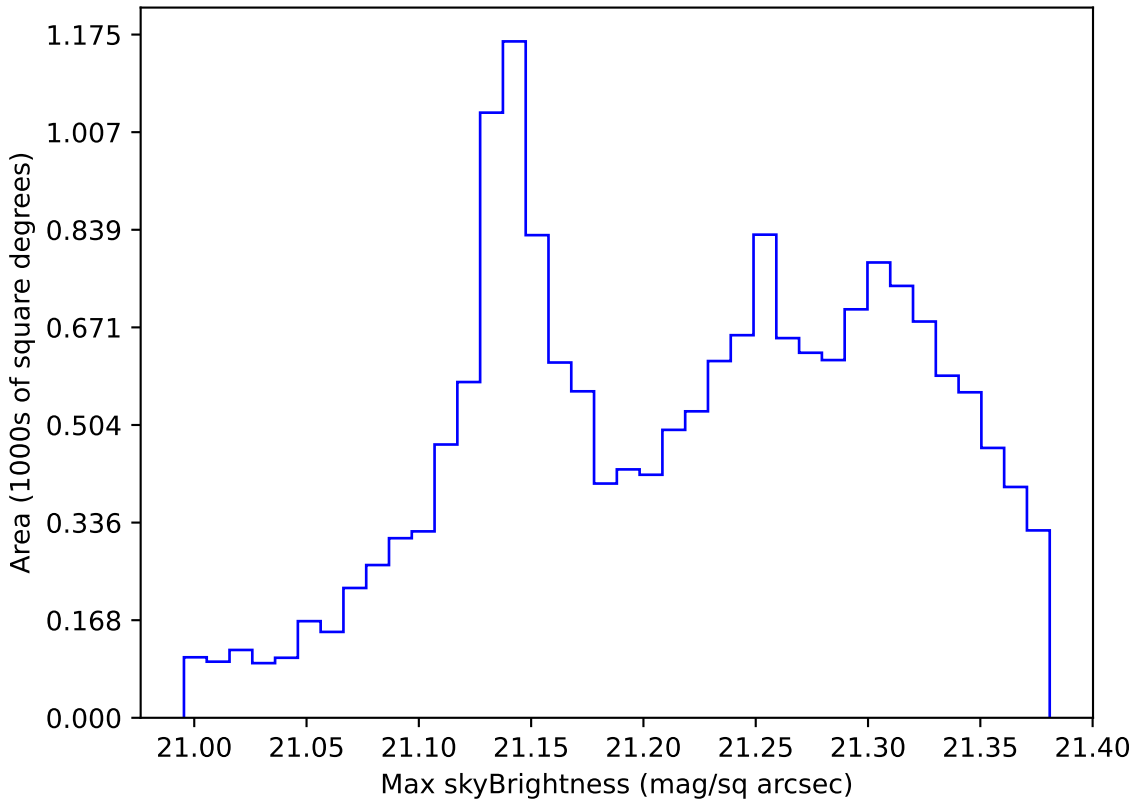
weather_cloudso30v3.4_10yrs WFD r band: Max skyBrightness
