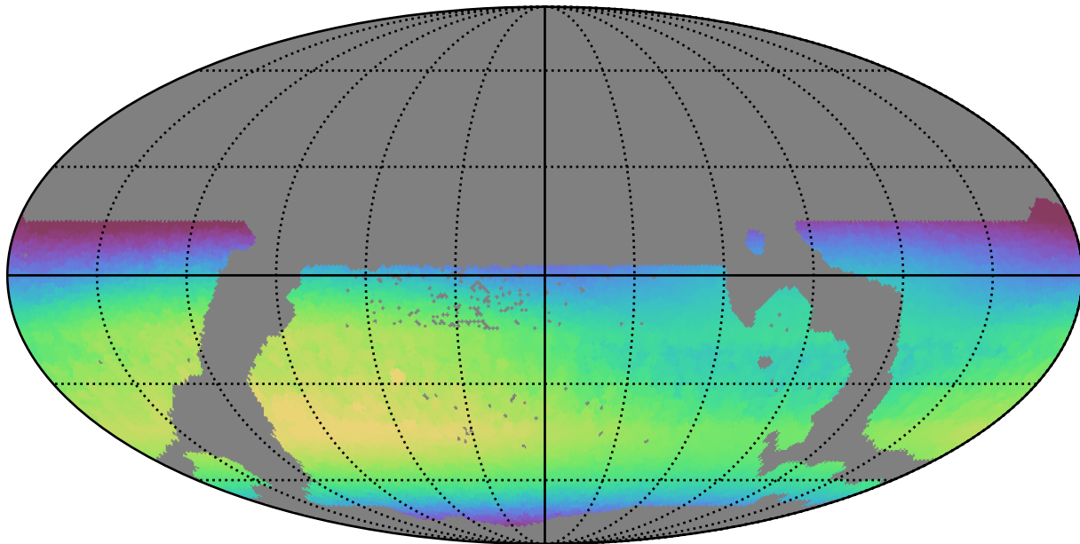
weather_cloudso30v3.4_10yrs WFD i band: Max skyBrightness
