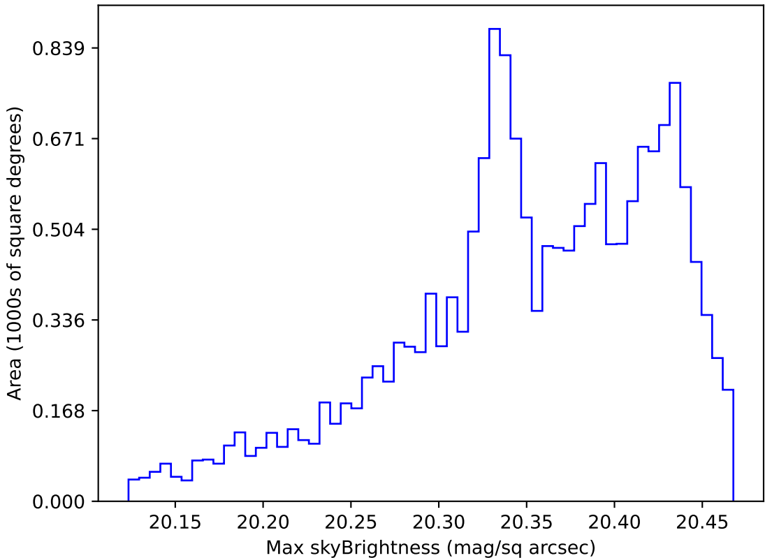
weather_cloudso30v3.4_10yrs WFD i band: Max skyBrightness
