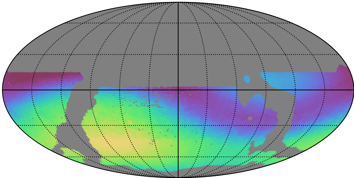
weather_cloudso30v3.4_10yrs WFD g band: Max skyBrightness
