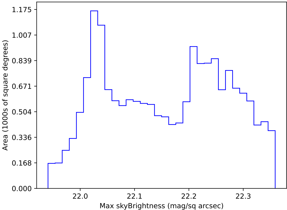
weather_cloudso30v3.4_10yrs WFD g band: Max skyBrightness
