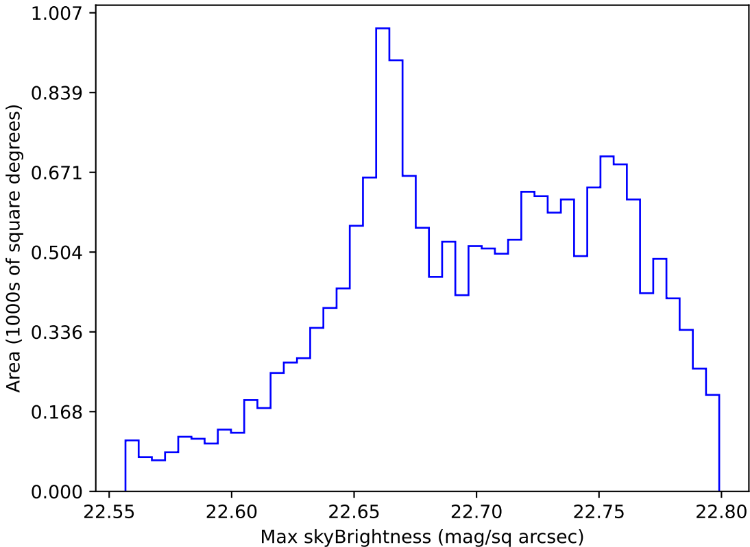
weather_cloudso30v3.4_10yrs WFD all bands: Max skyBrightness
