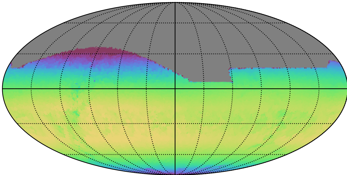
weather_cloudso30v3.4_10yrs All sky z band: Max skyBrightness
