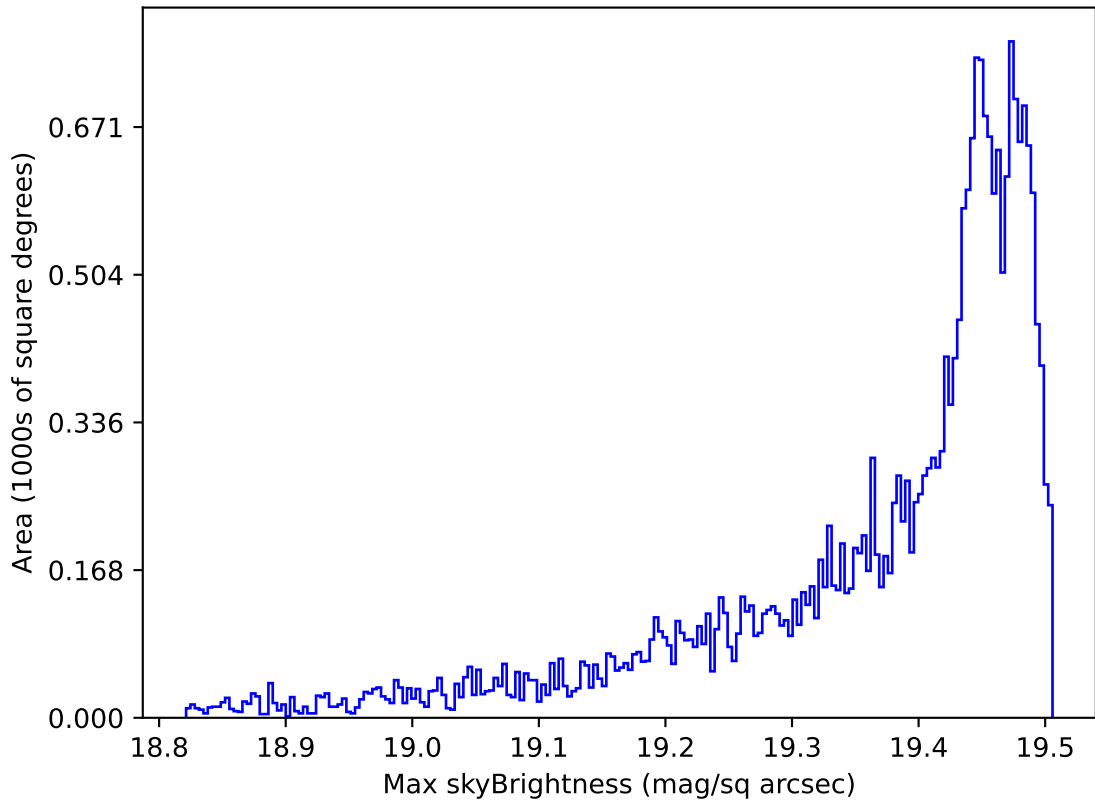
weather_cloudso30v3.4_10yrs All sky z band: Max skyBrightness
