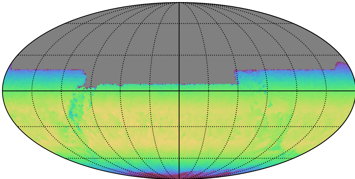
weather_cloudso30v3.4_10yrs All sky y band: Max skyBrightness
