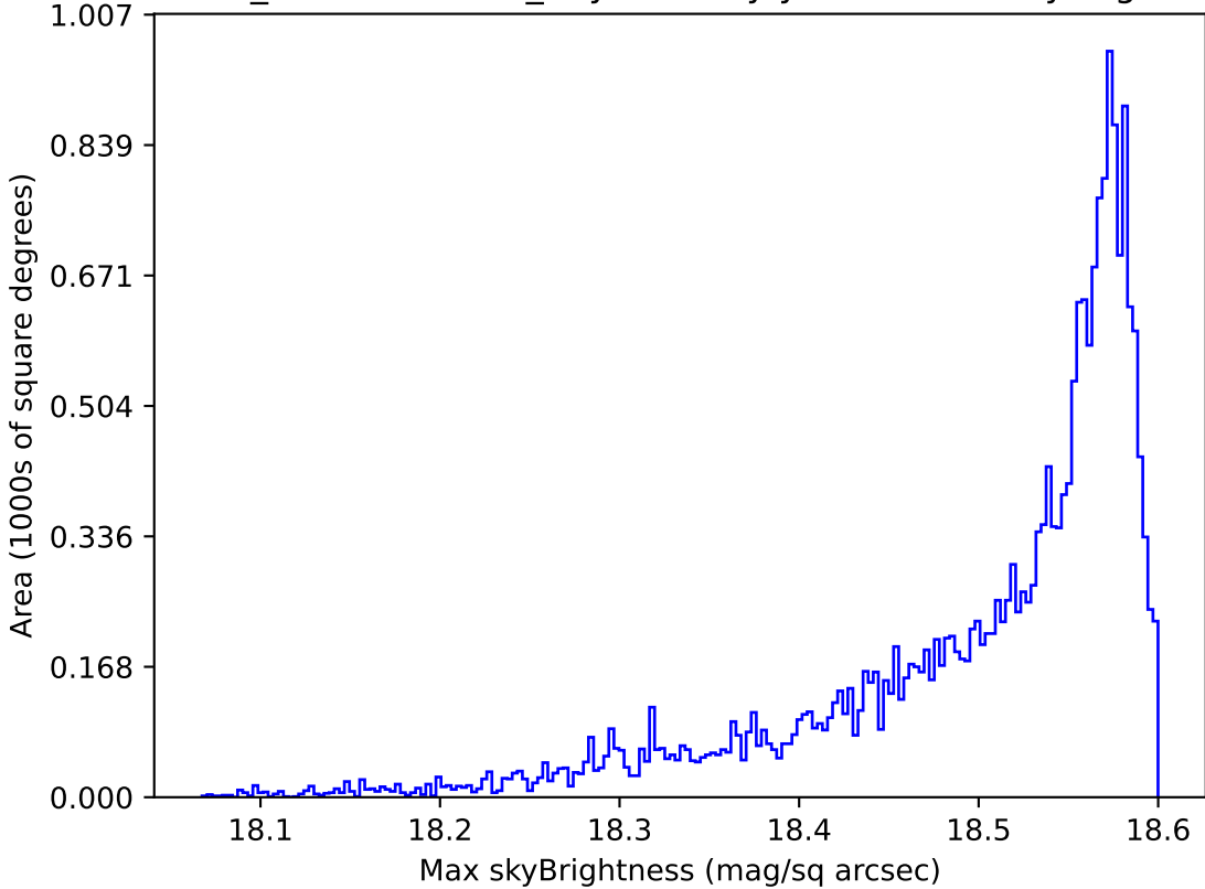
weather_cloudso30v3.4_10yrs All sky y band: Max skyBrightness
