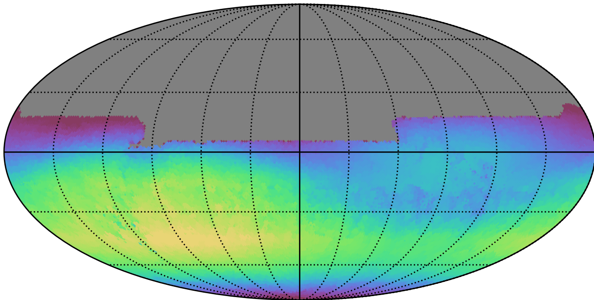
weather_cloudso30v3.4_10yrs All sky u band: Max skyBrightness
