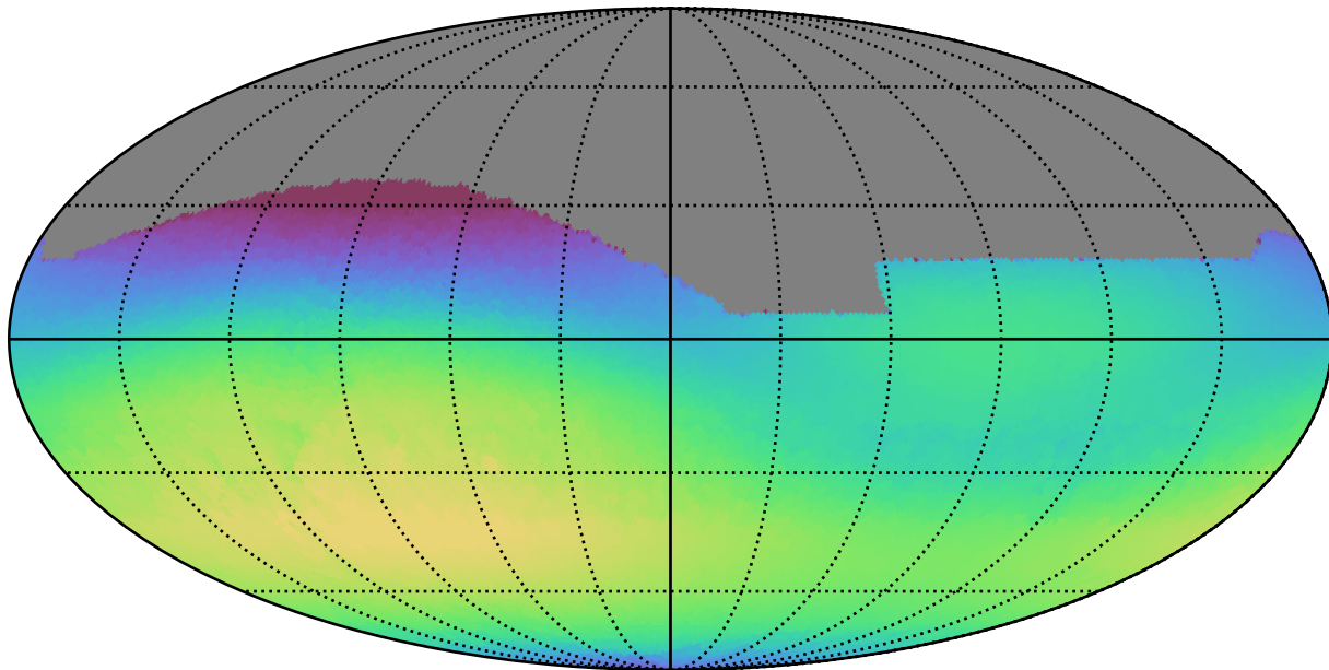
weather_cloudso30v3.4_10yrs All sky r band: Max skyBrightness
