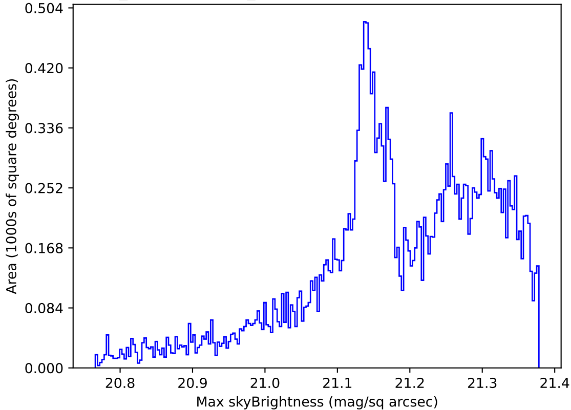
weather_cloudso30v3.4_10yrs All sky r band: Max skyBrightness
