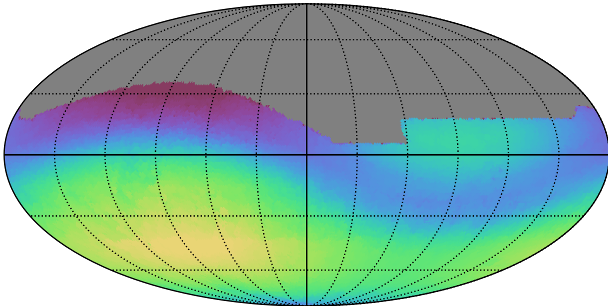
weather_cloudso30v3.4_10yrs All sky g band: Max skyBrightness
