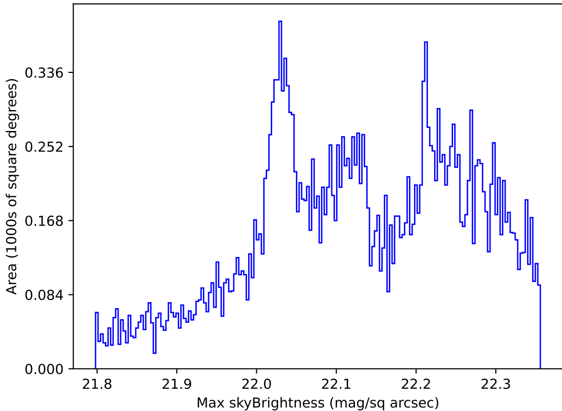
weather_cloudso30v3.4_10yrs All sky g band: Max skyBrightness
