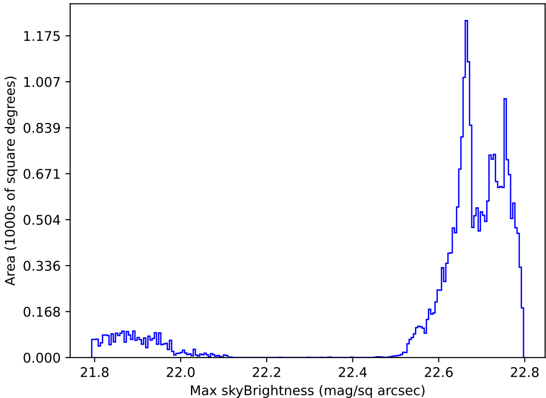
weather_cloudso30v3.4_10yrs All sky all bands: Max skyBrightness
