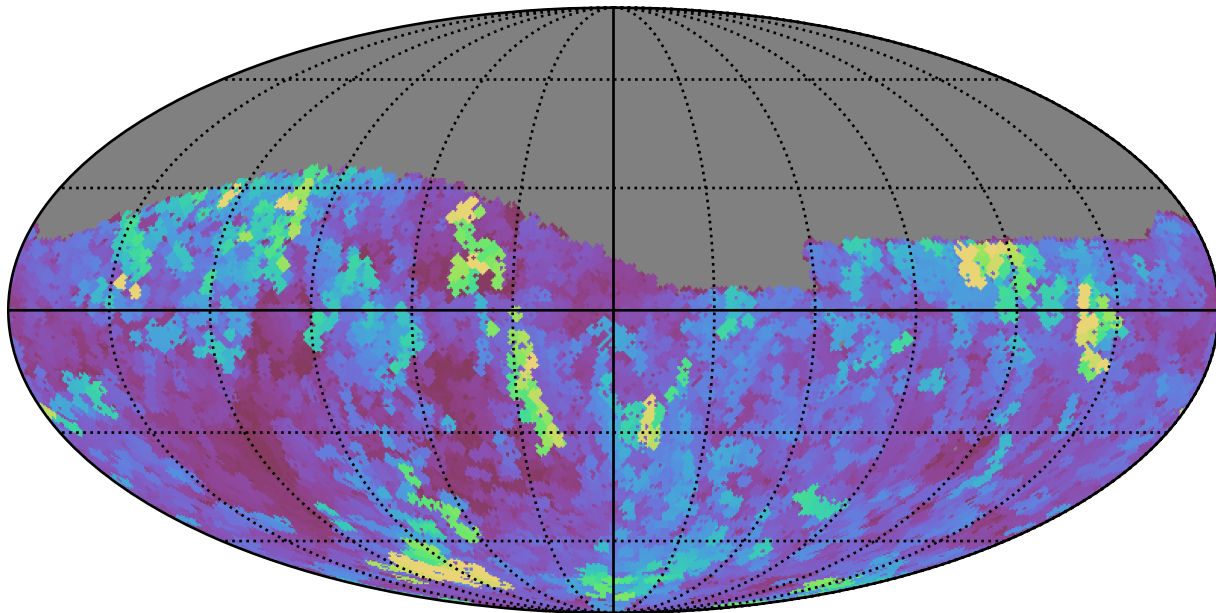
weather_cloudso30v3.4_10yrs Yr 1 z band: Max seeingGeom
