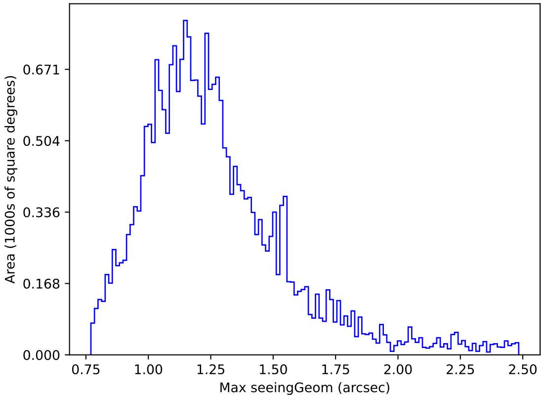
weather_cloudso30v3.4_10yrs Yr 1 z band: Max seeingGeom
