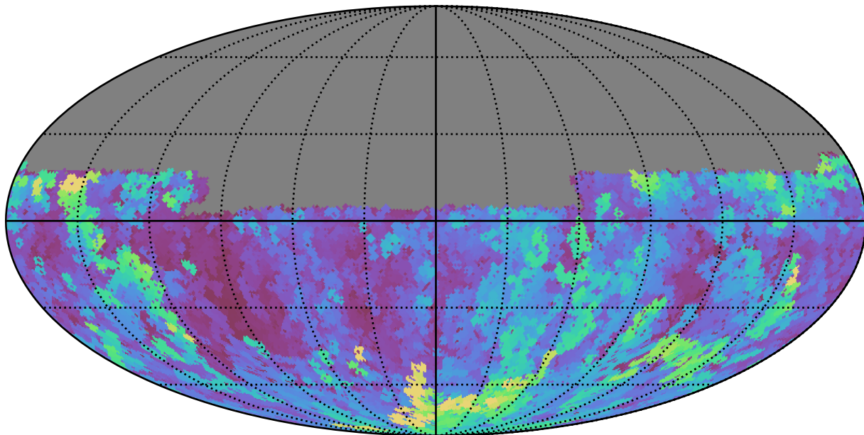
weather_cloudso30v3.4_10yrs Yr 1 u band: Max seeingGeom
