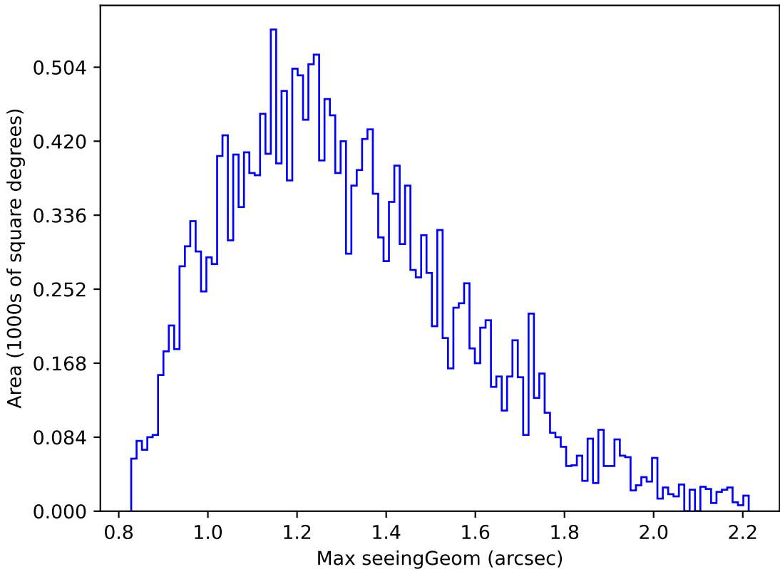
weather_cloudso30v3.4_10yrs Yr 1 u band: Max seeingGeom
