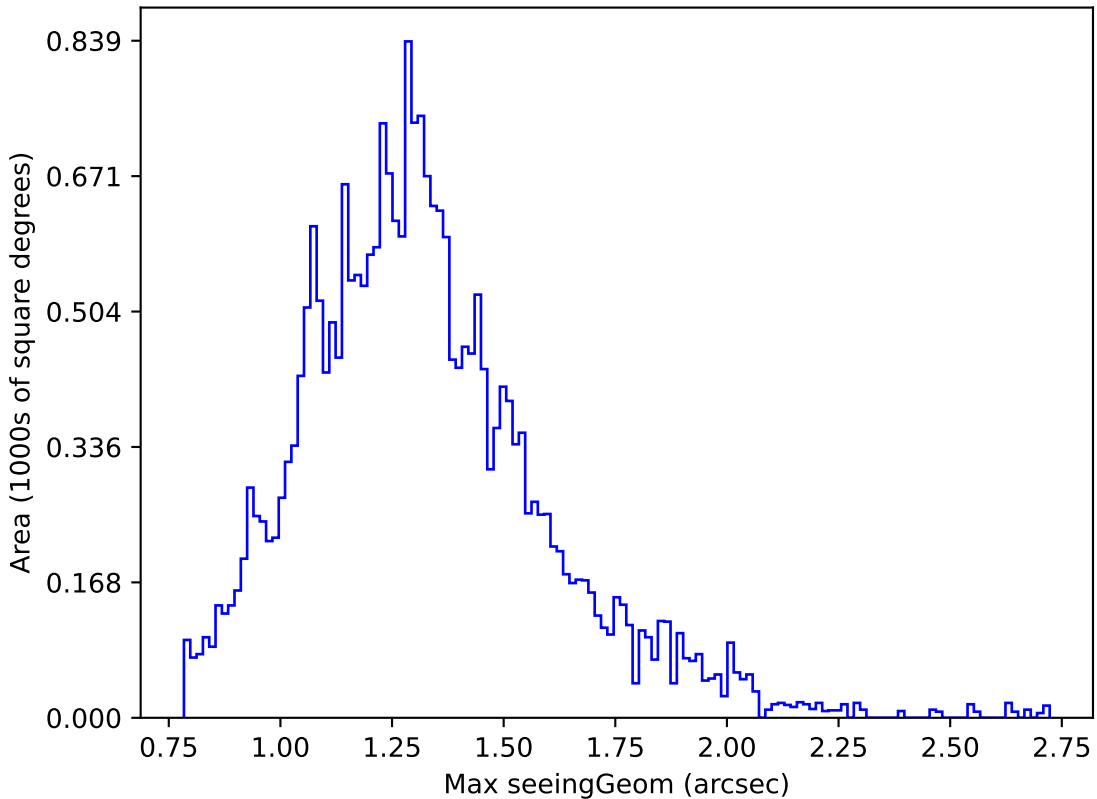
weather_cloudso30v3.4_10yrs Yr 1 r band: Max seeingGeom
