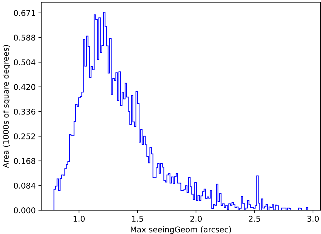
weather_cloudso30v3.4_10yrs Yr 1 i band: Max seeingGeom
