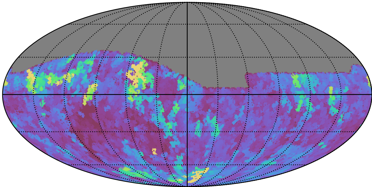
weather_cloudso30v3.4_10yrs Yr 1 all bands: Max seeingGeom
