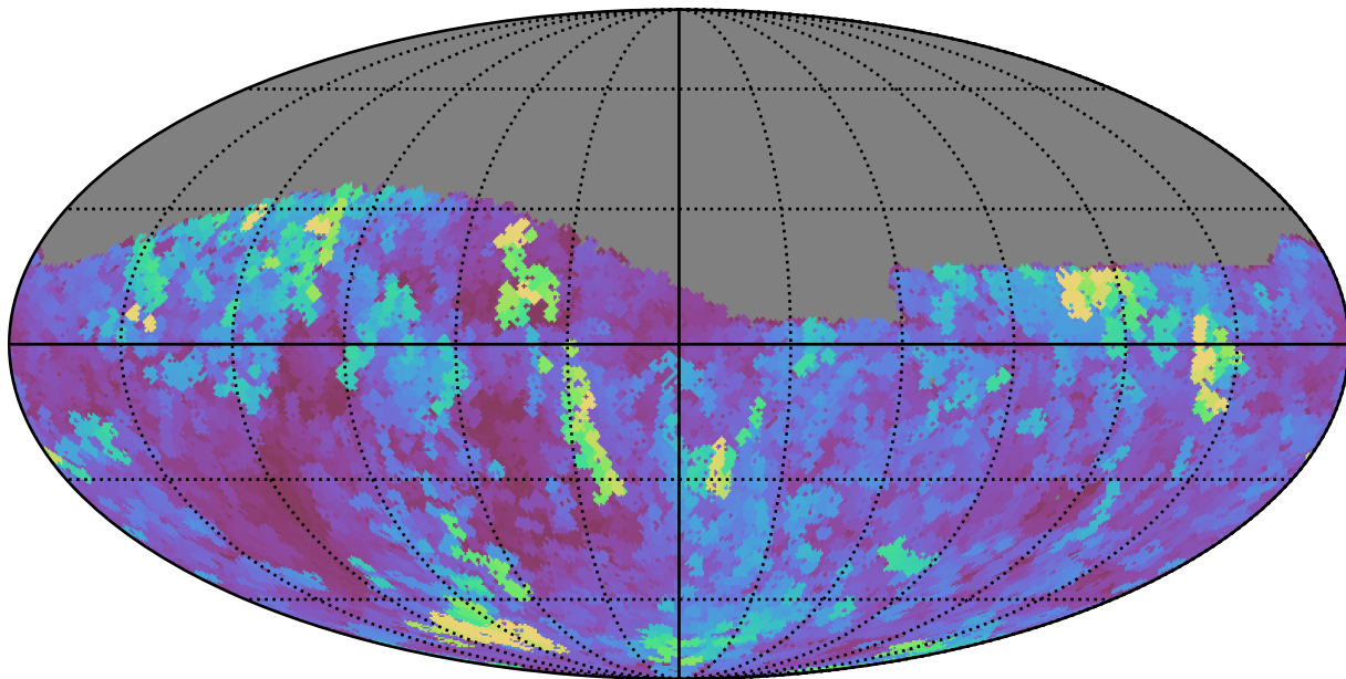
weather_cloudso30v3.4_10yrs Yr 1 z band: Max seeingEff
