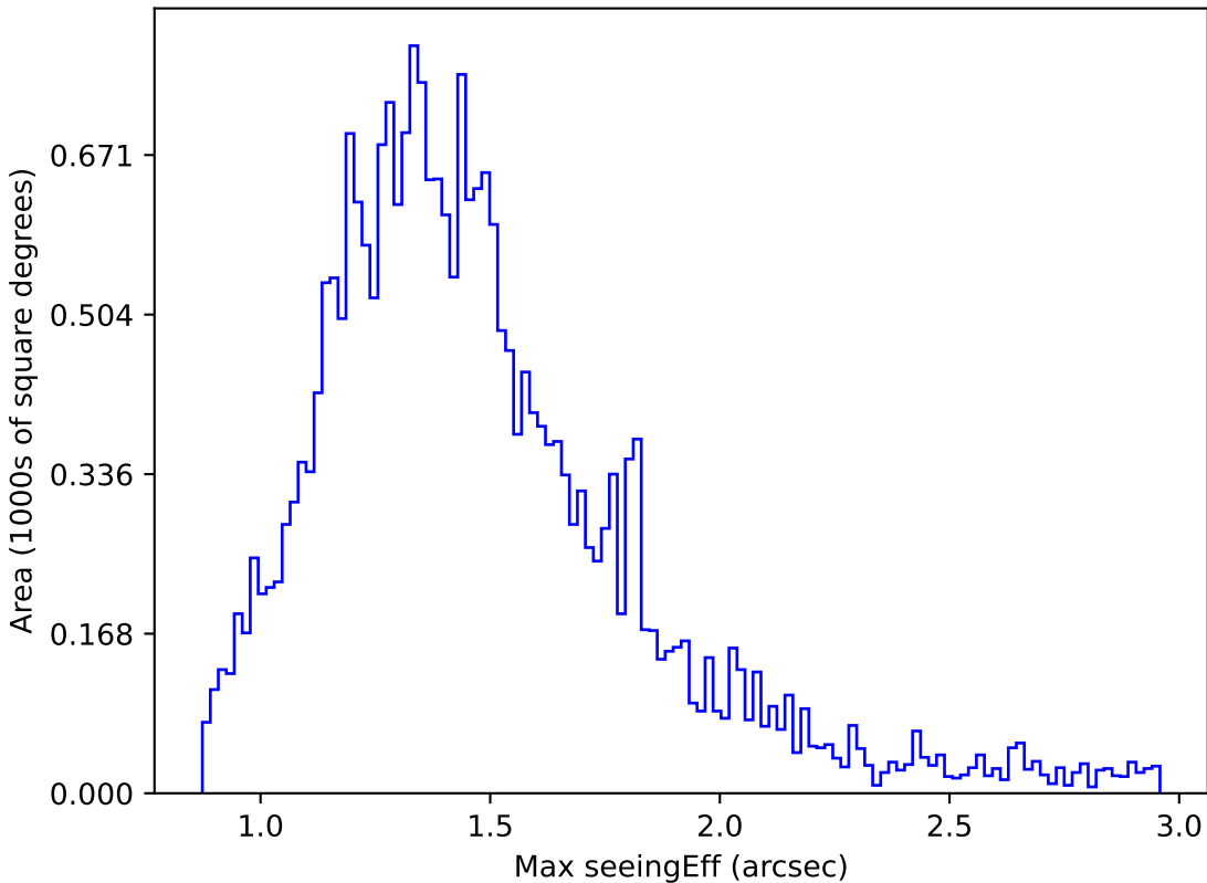
weather_cloudso30v3.4_10yrs Yr 1 z band: Max seeingEff
