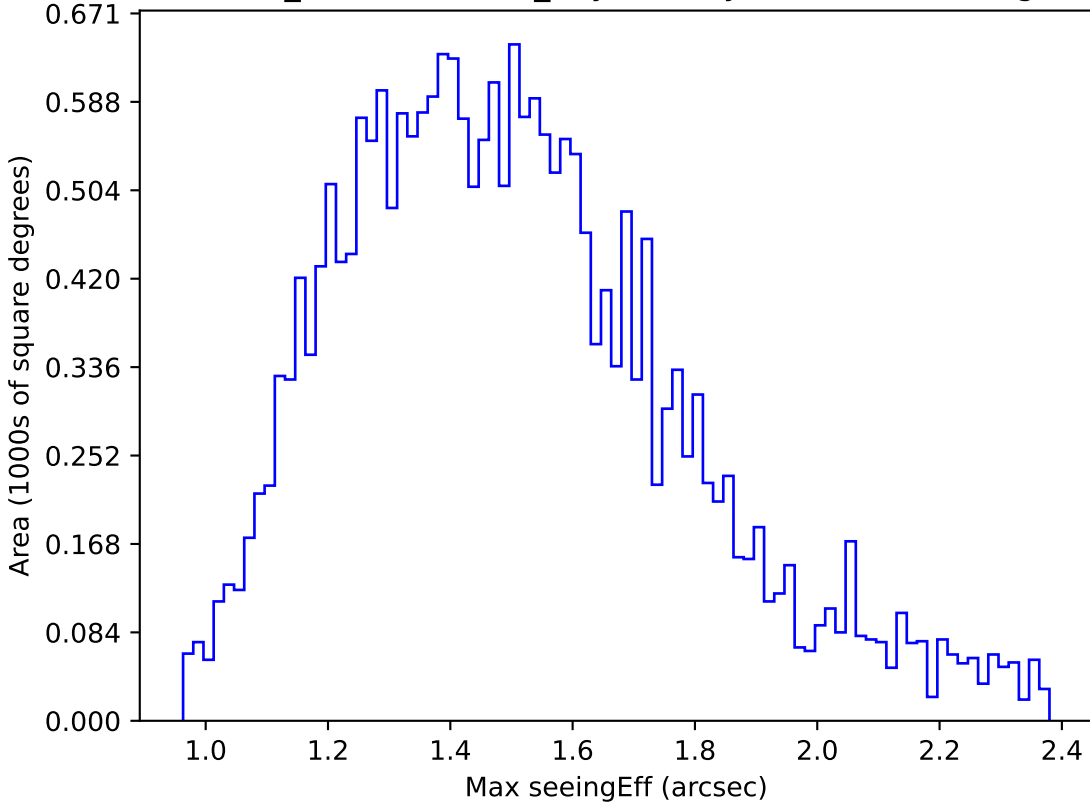
weather_cloudso30v3.4_10yrs Yr 1 y band: Max seeingEff
