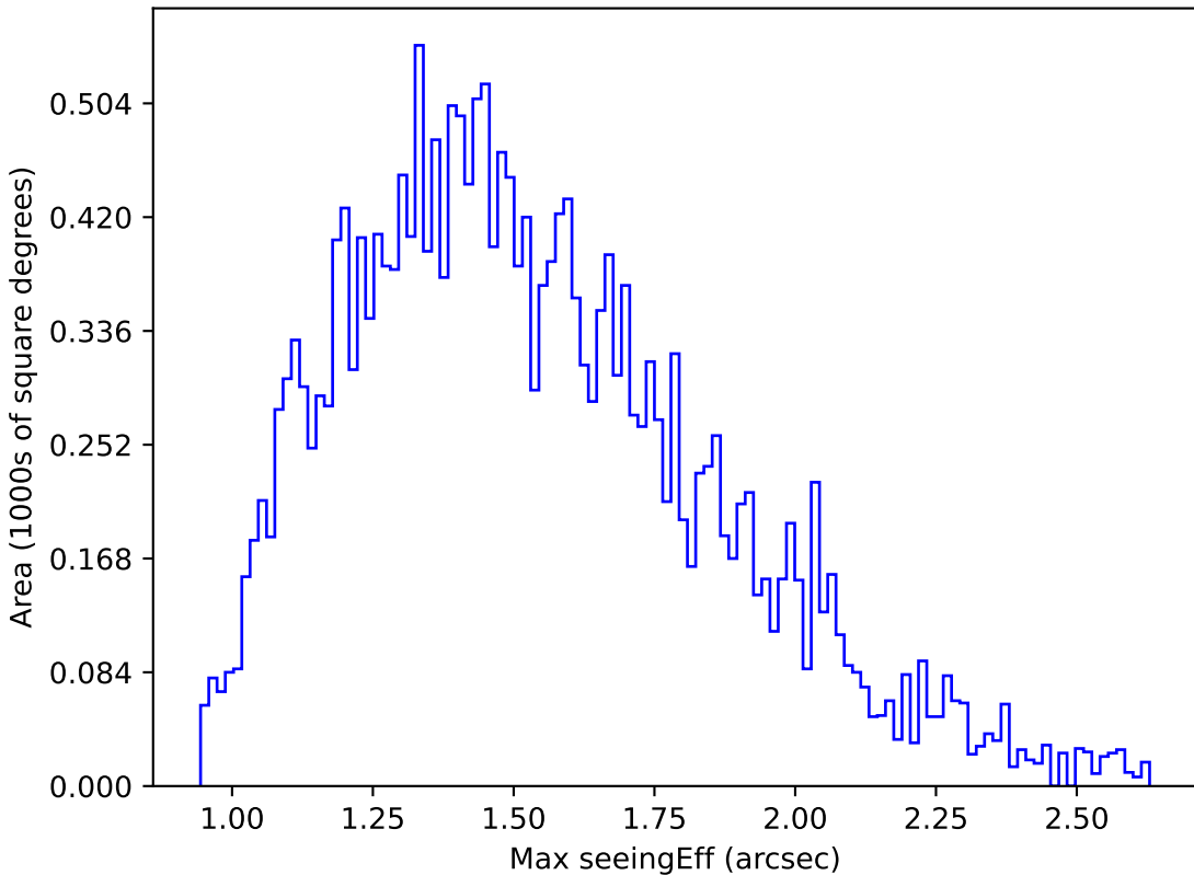
weather_cloudso30v3.4_10yrs Yr 1 u band: Max seeingEff
