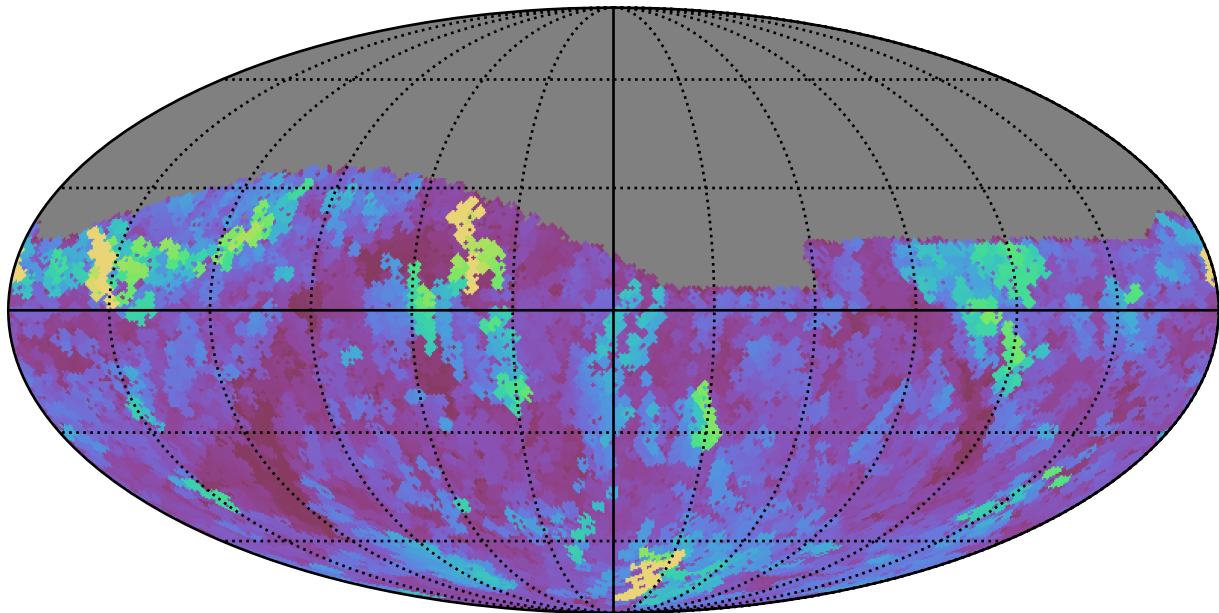
weather_cloudso30v3.4_10yrs Yr 1 i band: Max seeingEff
