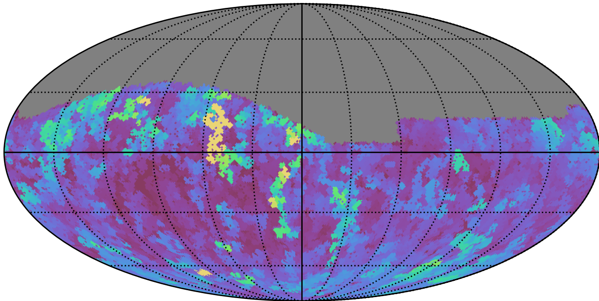
weather_cloudso30v3.4_10yrs Yr 1 g band: Max seeingEff
