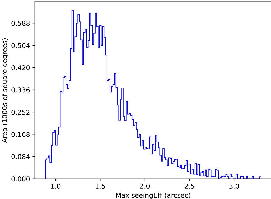
weather_cloudso30v3.4_10yrs Yr 1 g band: Max seeingEff
