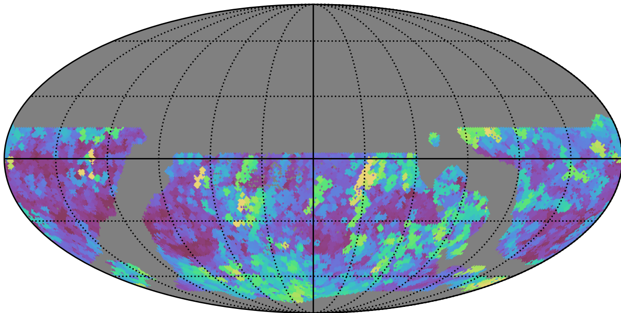
weather_cloudso30v3.4_10yrs WFD r band: Max seeingEff
