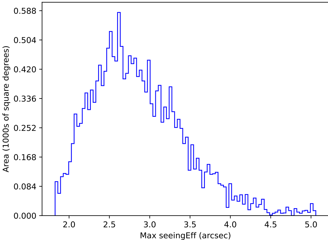
weather_cloudso30v3.4_10yrs WFD i band: Max seeingEff
