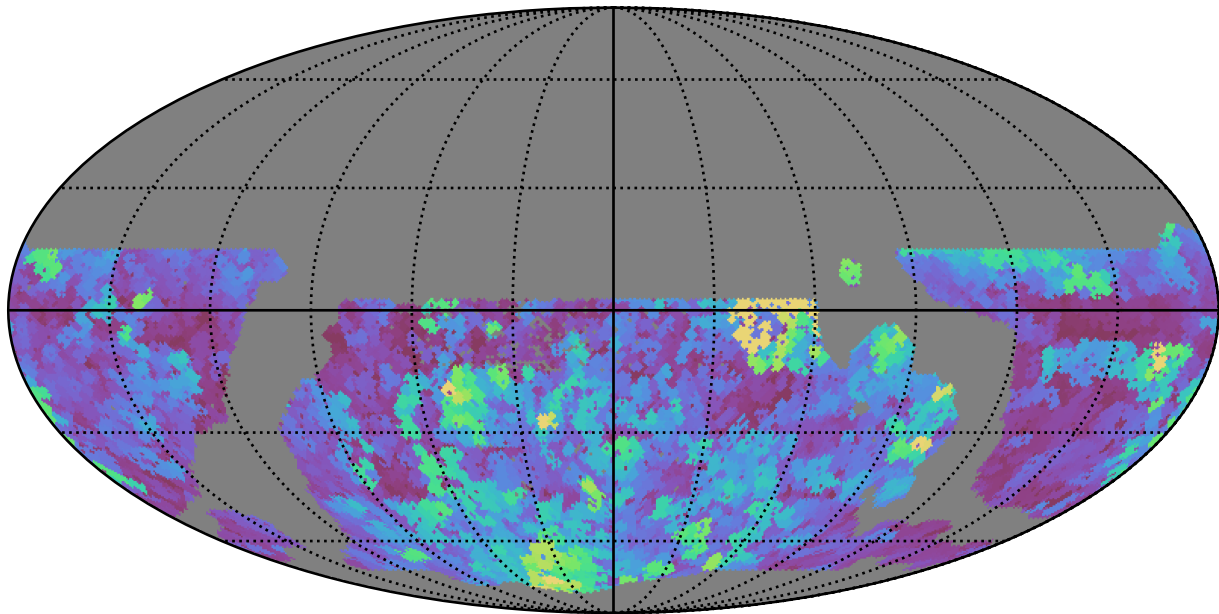
weather_cloudso30v3.4_10yrs WFD g band: Max seeingEff
