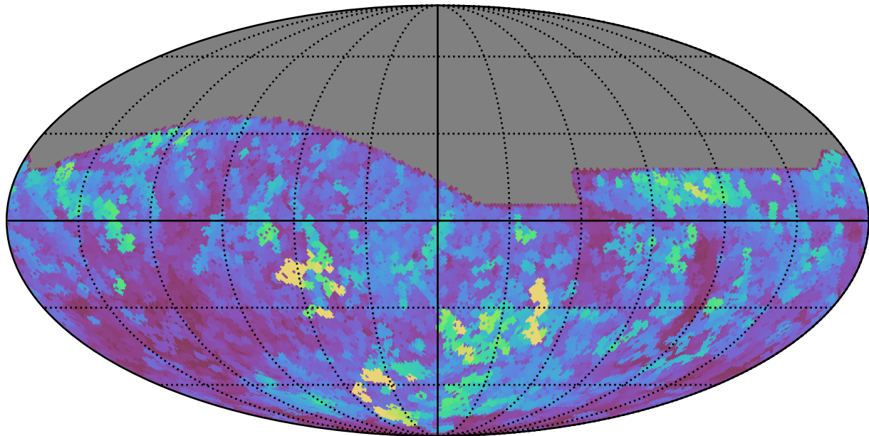
weather_cloudso30v3.4_10yrs All sky z band: Max seeingEff
