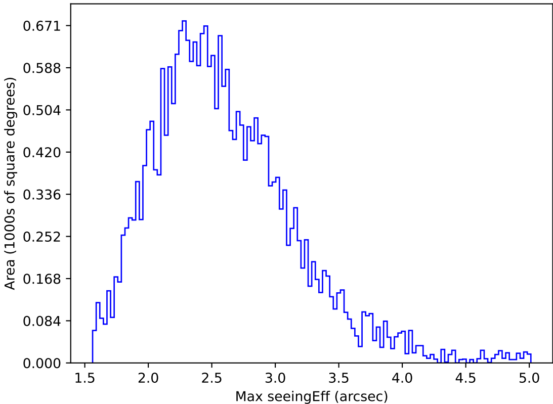
weather_cloudso30v3.4_10yrs All sky z band: Max seeingEff
