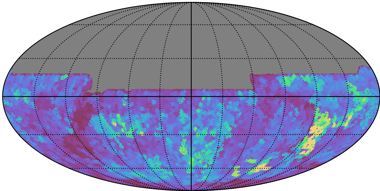
weather_cloudso30v3.4_10yrs All sky y band: Max seeingEff
