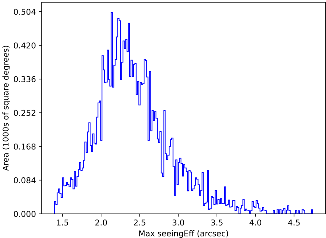
weather_cloudso30v3.4_10yrs All sky y band: Max seeingEff
