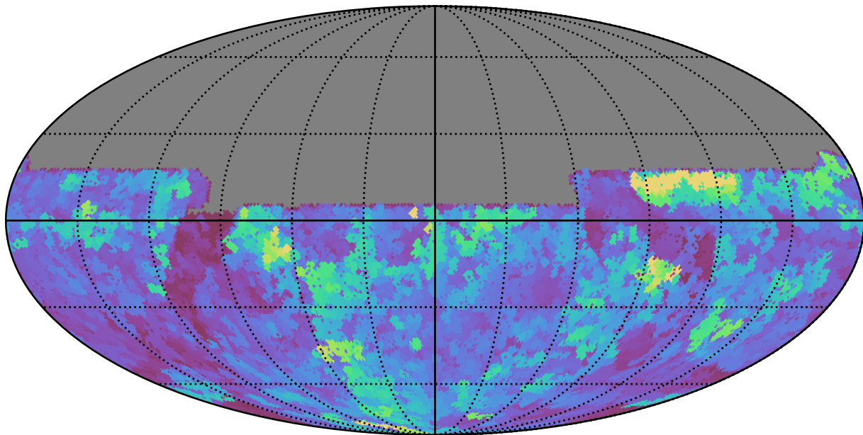
weather_cloudso30v3.4_10yrs All sky u band: Max seeingEff
