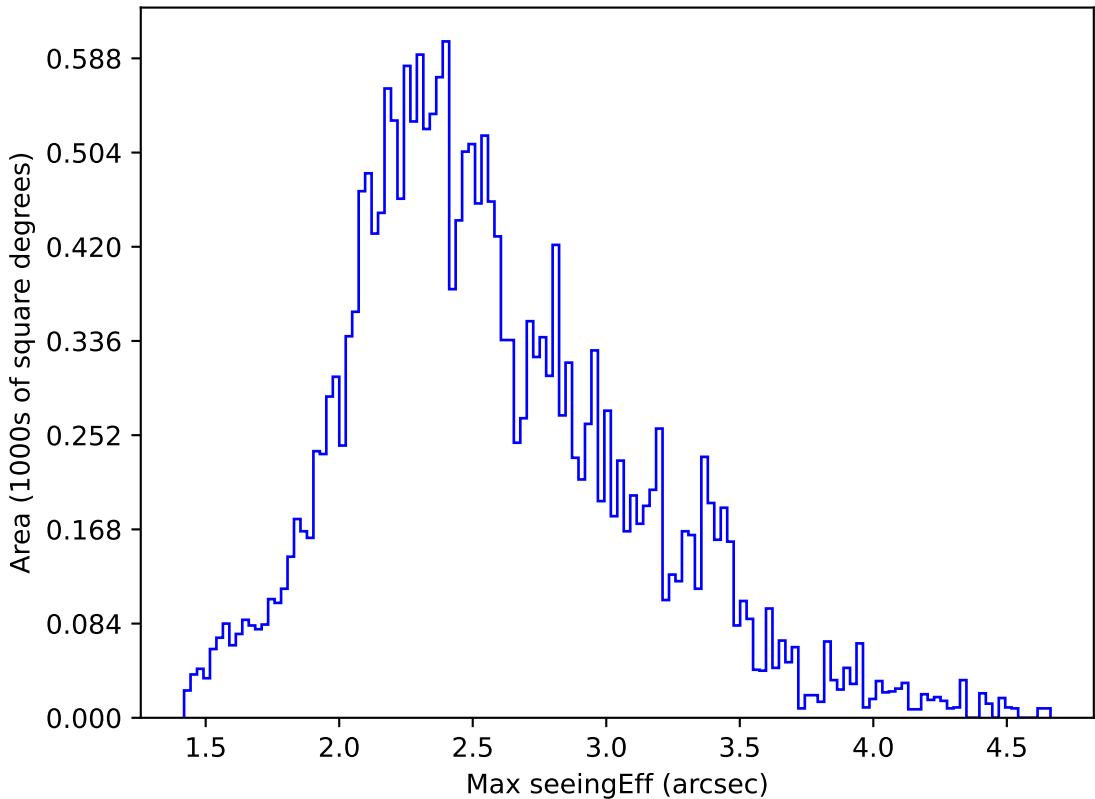
weather_cloudso30v3.4_10yrs All sky u band: Max seeingEff
