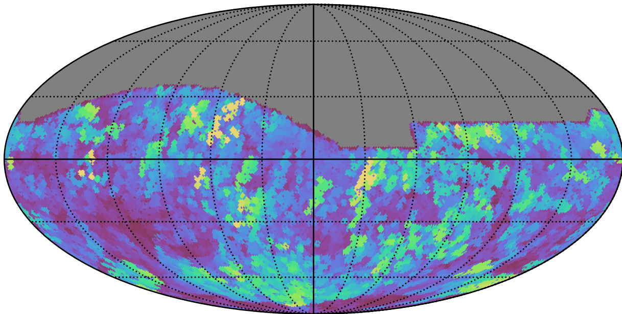
weather_cloudso30v3.4_10yrs All sky r band: Max seeingEff
