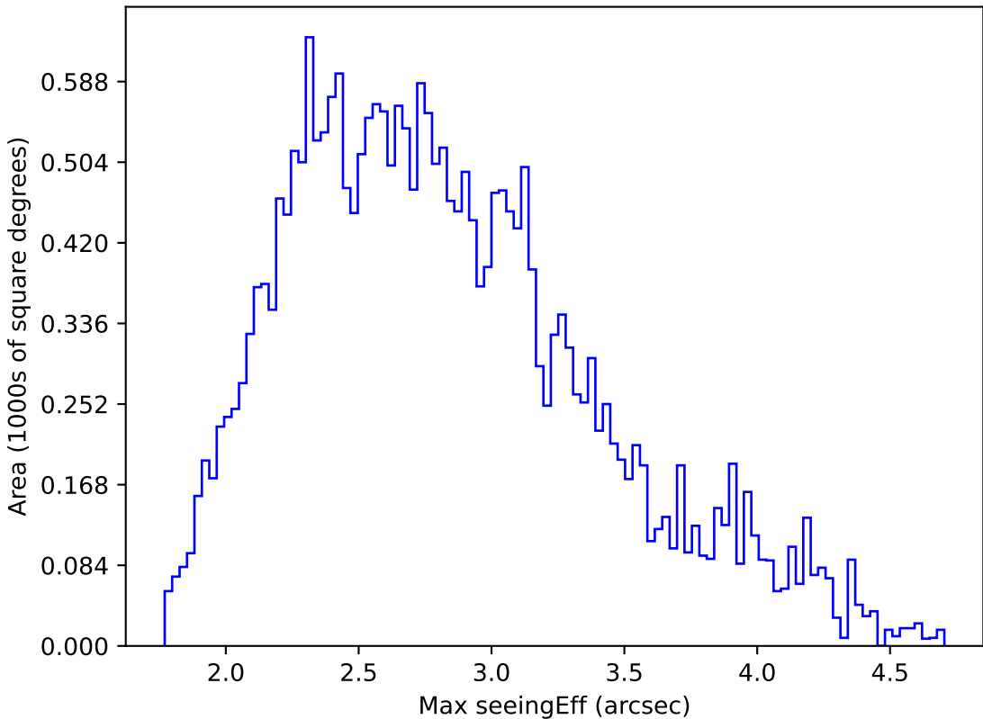
weather_cloudso30v3.4_10yrs All sky r band: Max seeingEff
