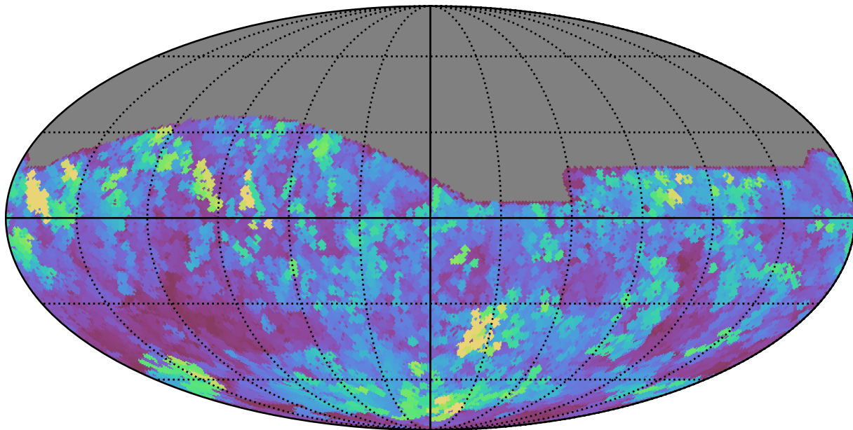
weather_cloudso30v3.4_10yrs All sky i band: Max seeingEff
