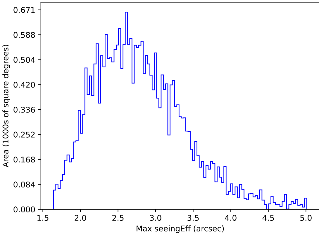
weather_cloudso30v3.4_10yrs All sky i band: Max seeingEff
