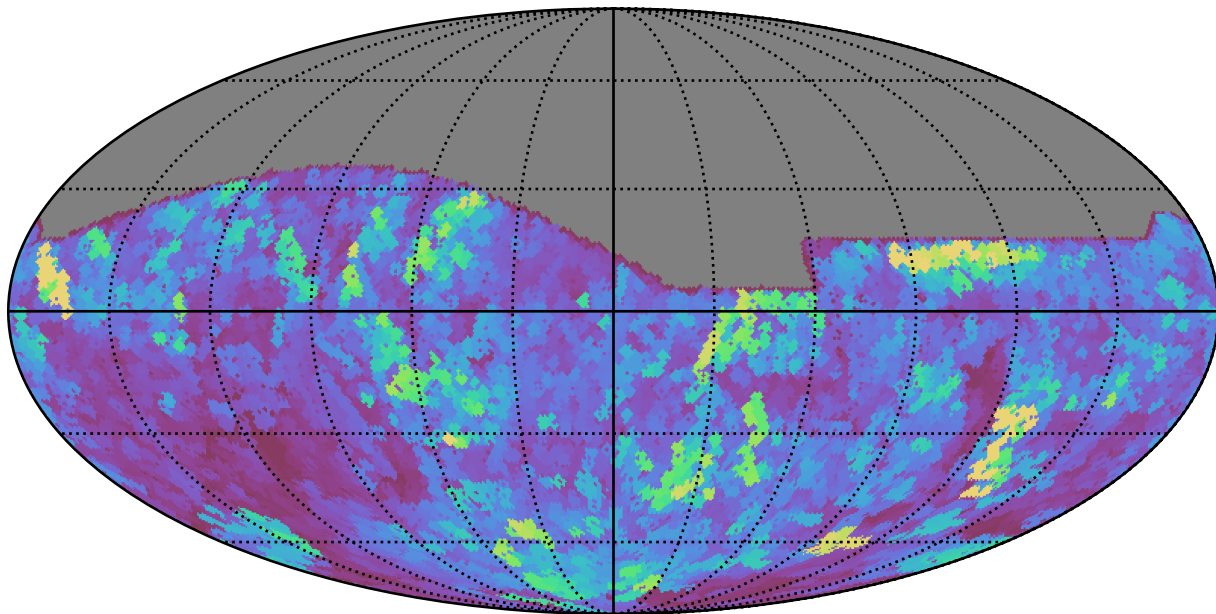
weather_cloudso30v3.4_10yrs All sky all bands: Max seeingEff
