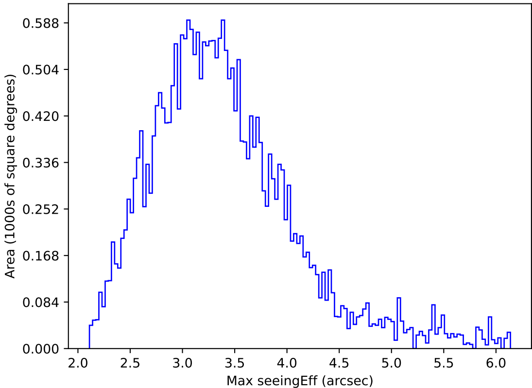
weather_cloudso30v3.4_10yrs All sky all bands: Max seeingEff
