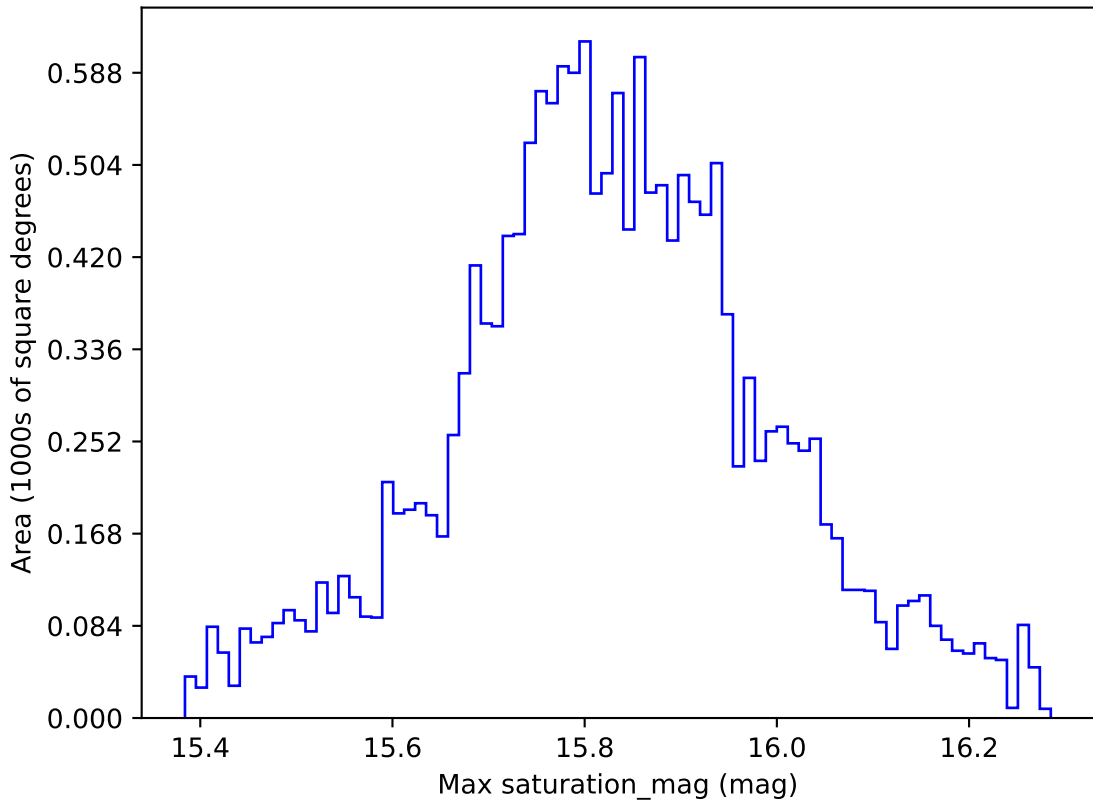
weather_cloudso30v3.4_10yrs WFD all bands: Max saturation_mag
