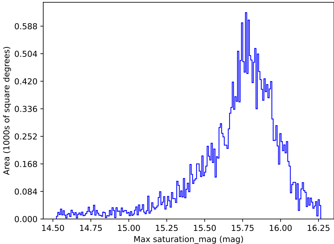
weather_cloudso30v3.4_10yrs All sky all bands: Max saturation_mag
