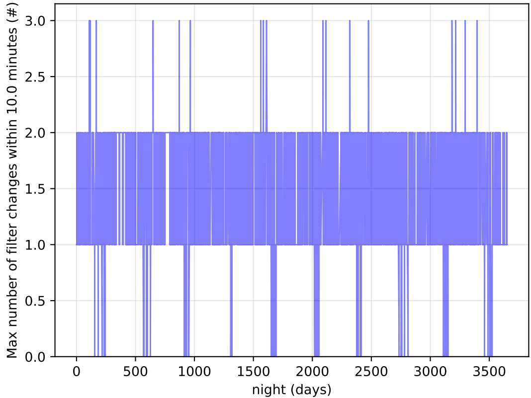
weather_cloudso30v3.4_10yrs Per Night: Max number of filter changes within 10.0 minutes
