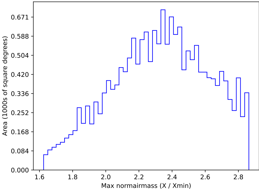
weather_cloudso30v3.4_10yrs WFD z band: Max normairmass
